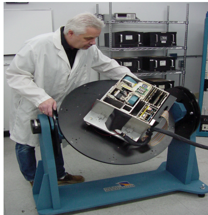
Navhouse Honeywell IRS Test Stand
